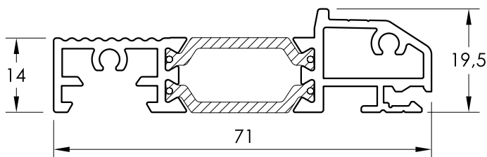
PM 090 UMBRAL IT-71-NG
