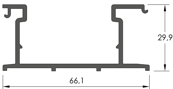
AH 45854 - Poliamida
