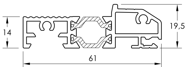
PF 090 UMBRAL IT-61-NG
