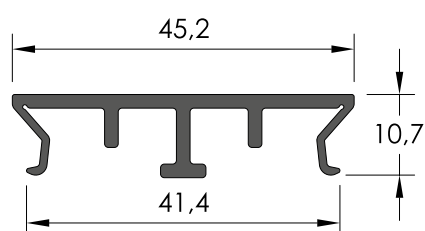
AH 45813 - Poliamida
