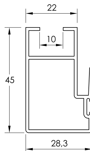
27163 HOJA CENTRAL
