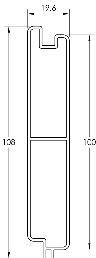
64781 LAMA PORTAL
