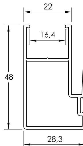
27163 HOJA CENTRAL
