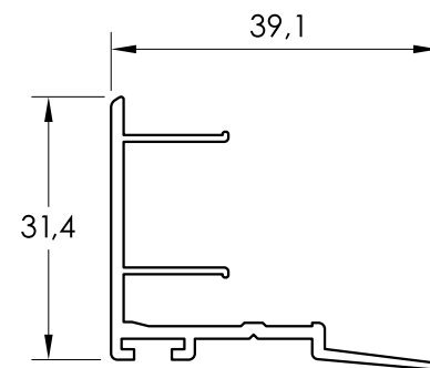
24145 ENGANCHE CENTRAL
